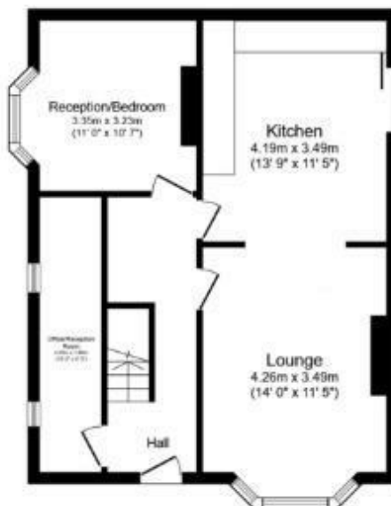
Ground Floor Floor area 57.6 sq.m. (620 sq.ft.)
